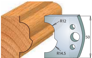
Pair of knives 690.519 Pair of limiters 691.519
