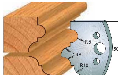
Pair of knives 690.520 Pair of limiters 691.520
