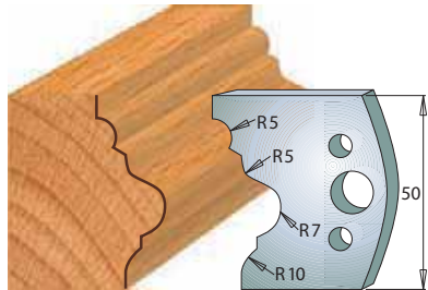
Pair of knives 690.508 Pair of limiters 691.508
