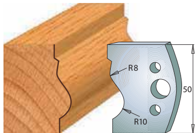
Pair of knives 690.510 Pair of limiters 691.510
