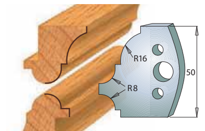
Pair of knives 690.541 Pair of limiters 691.541
