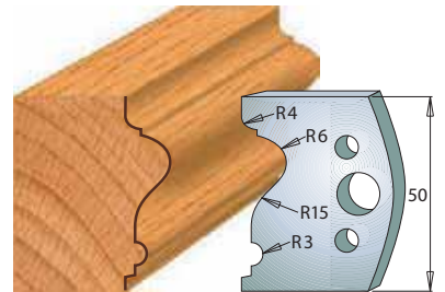
Pair of knives 690.512 Pair of limiters 691.512
