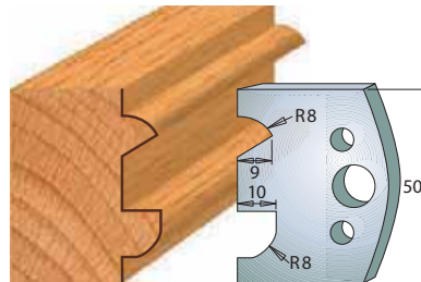
Pair of knives 690.517 Pair of limiters 691.517
