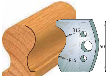
Pair of knives 690.514 Pair of limiters 691.514
