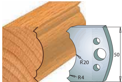
Pair of knives 690.507 Pair of limiters 691.507
