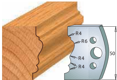
Pair of knives 690.511 Pair of limiters 691.511
