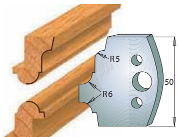
Pair of knives 690.542 Pair of limiters 691.542
