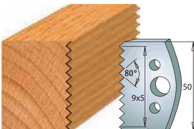
Pair of knives 690.524 Pair of limiters 691.524
