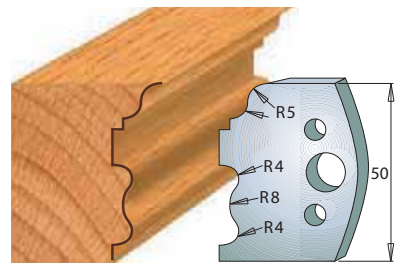
Pair of knives 690.515 Pair of limiters 691.515
